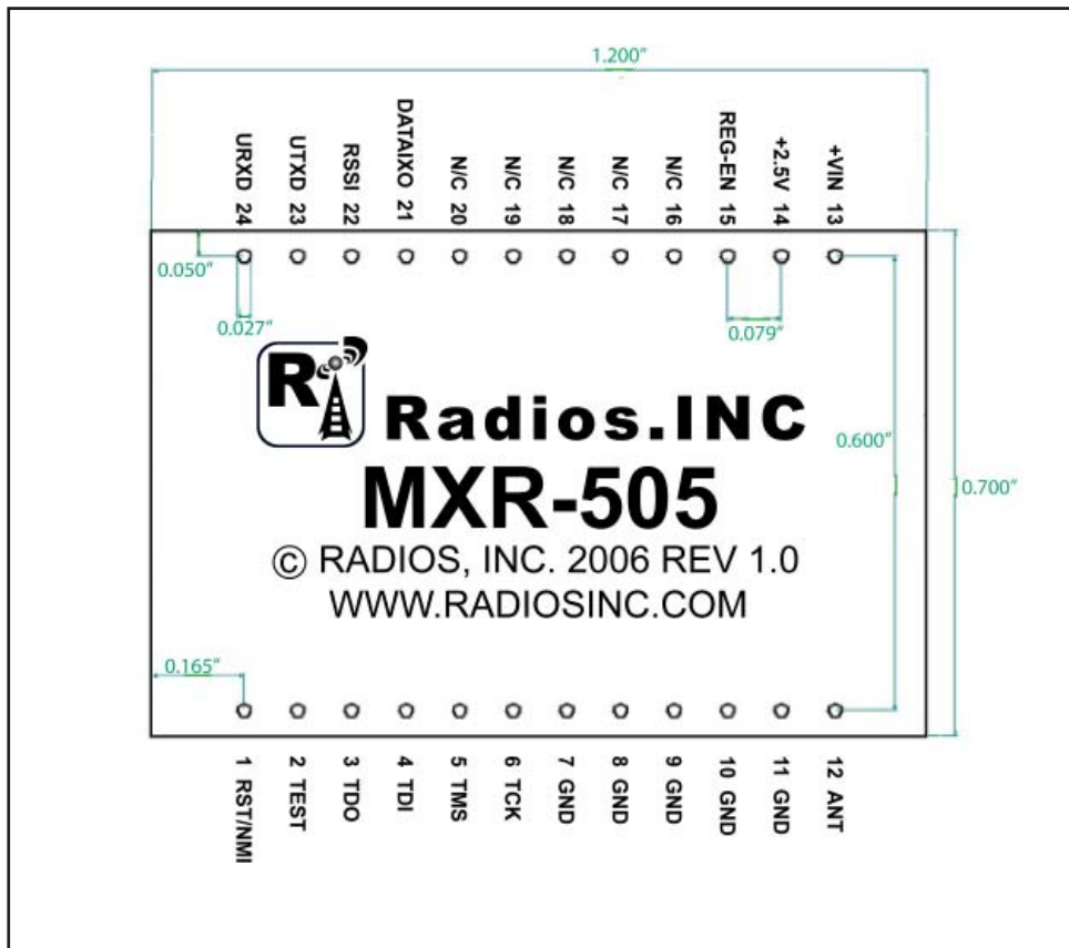
DIP Package
